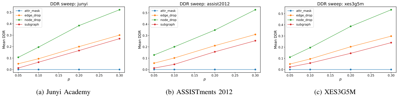
Fig. 4: DDR as a function of perturbation strength p for four label-agnostic graph augmentation families across three datasets. Each marker plots the mean DDR averaged across nine stochastic runs (three random seeds on each of three train folds). Across all datasets the four families separate into four distinct regimes: \text{DDR}(\text{attr\_mask}) = 0 < \text{DDR}(\text{subgraph}) < \text{DDR}(\text{edge\_drop}) \approx p < \text{DDR}(\text{node\_drop}) .
