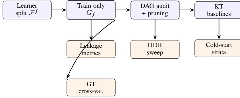
Fig. 2: Research framework connecting protocol modules (Section III) and experiment tracks (Section IV). Strengths: fold-conditioned provenance, explicit DAG repair, structural diagnostics decoupled from AUC, optional expert cross-validation. Limitations: fixed behavioural inference rule; similarity rule fails on single-skill Q-matrices; DDR covers only four generic augmentations; GT CV available only where expert graphs exist.
