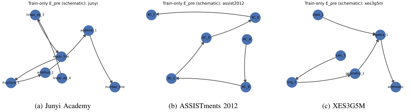
Fig. 3: Schematic visualisations of high-support prerequisite chains in train-only E_{\text{pre}} after DAG audit (representative subgraphs for interpretation; full graphs contain hundreds to thousands of edges). Junyi retains dense arithmetic progressions; ASSISTments and XES3G5M exhibit sparser chains consistent with Table IV.
